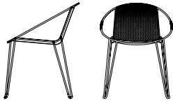
Dining Chair 560mm x 610mm x 760mm H (22in. x 24in. x 30in. H) (450mm/17.75in. seat height)
