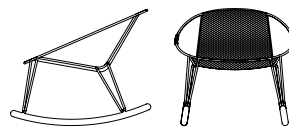
Rocker 670mm x 750mm x 660mm H (26.5in. x 29.5in. x 26in. H) (400mm/15.75in. seat height)
