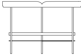
Coffee Table 600mm Dia x 400mm H (23.5in. Dia x 15.75in. H)
