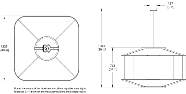
ALP-48-ST AllSew Pendant 48" Stem Dimension
