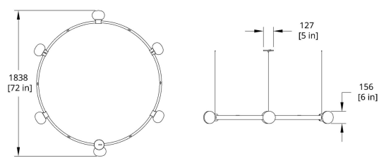
C6-6 Cinema Chandelier Dimension
