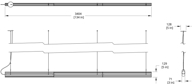
QP-44 Queue Pendant Dimension (Direct Indirect)
