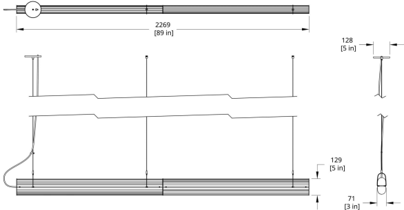
QP-88 Queue Pendant Dimension (Direct Indirect)
