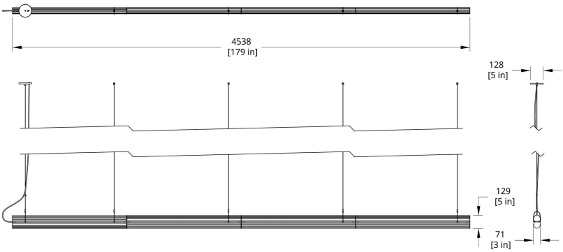
QP-88 Queue Pendant Dimension (Direct Indirect)
