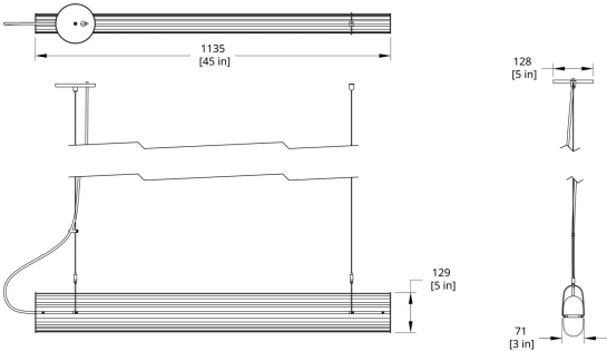
QP-44 Queue Pendant Dimension (Direct Indirect)
