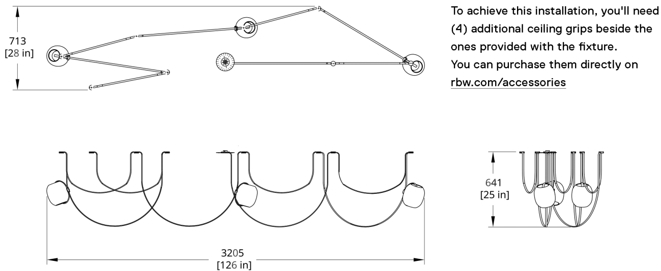
VS-3 Vitis Chandelier (Condensed High) Dimension
