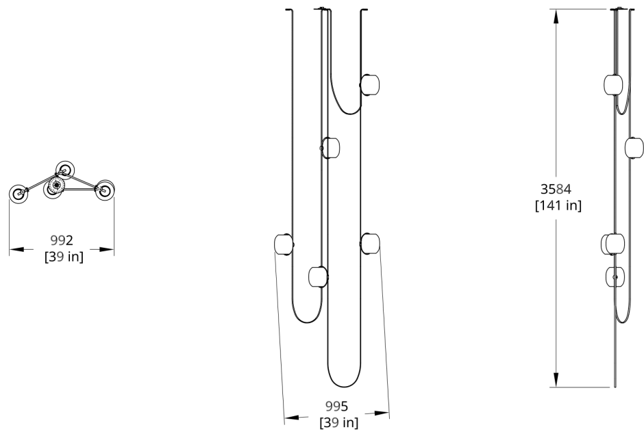
VS-5 Vitis Chandelier (Extra Long) Dimension
