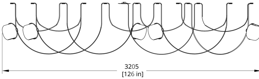
VS-5 Vitis Chandelier (High) Dimension
