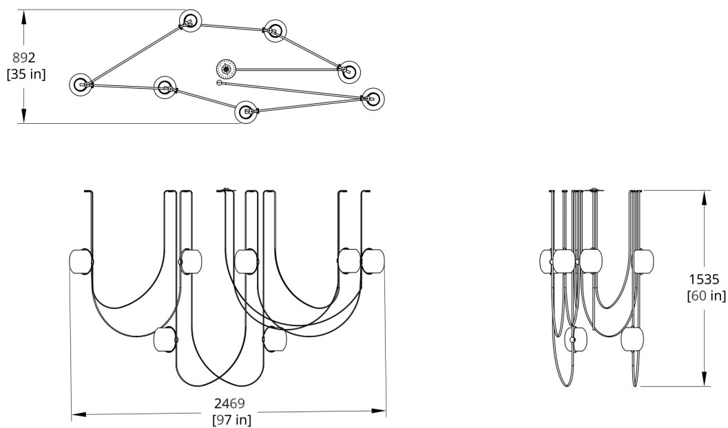
VS-7 Vitis Chandelier (Condensed) Dimension
