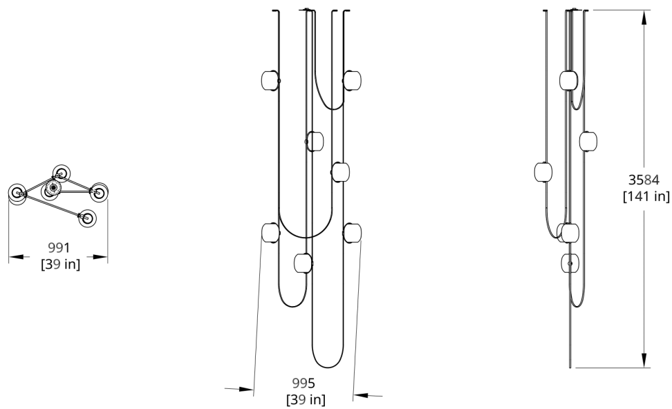
VS-7 Vitis Chandelier (Extra Long) Dimension
