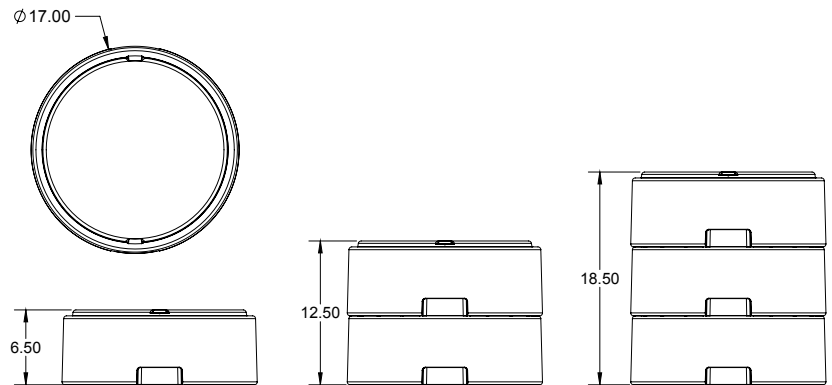
HEIGHT WITH ROCKER BASE DISENGAGED
