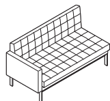
Overall: 30"D 55"W 31"H Inside: 22"D 52¾"W 17"H
