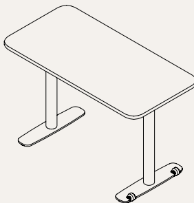
M / L / XL RECTANGLE Width: 1200mm, 1500mm, 1600mm, 1800mm, 2000mm, 2200mm Depth: 600mm (M), 750mm (L), 1050mm (XL)
