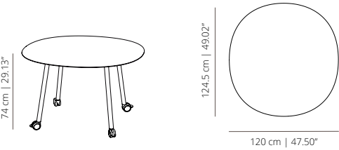
MAAD120 table 120 | 47 1 / 4 with casters
