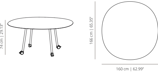
MAAD160 table 160 | 62 63 / 64 with casters
