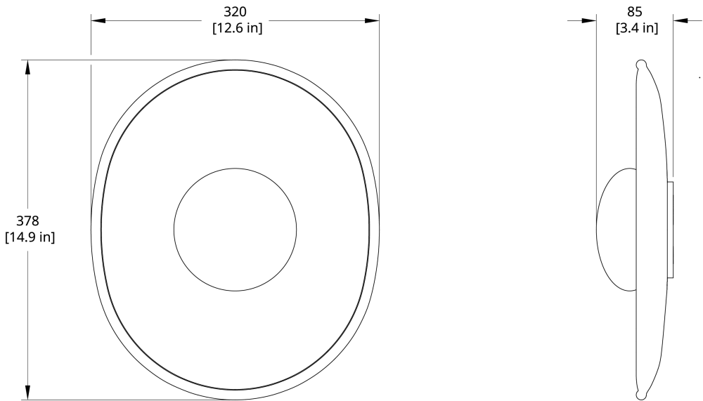
CP Crepe Medium Dimensional Drawing
