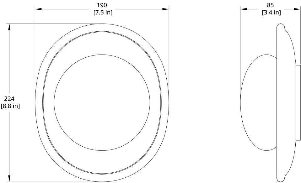
CP Crepe Small Dimensional Drawing
