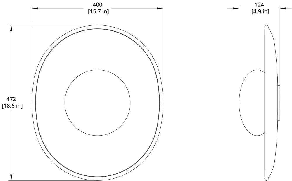
CP Crepe Large Dimensional Drawing
